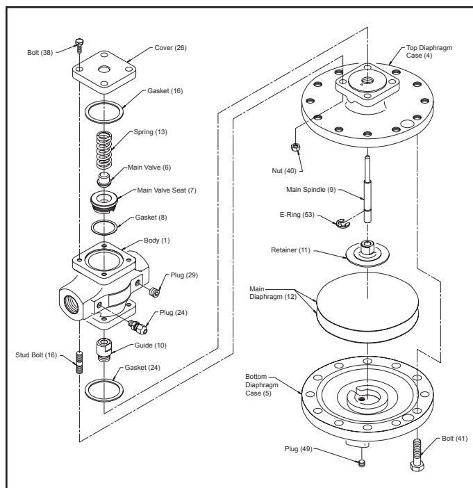
Figure 3-2. OB-2000 Main Valve
